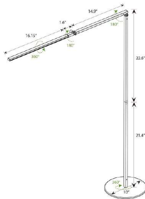
Horizontal and vertical reach
