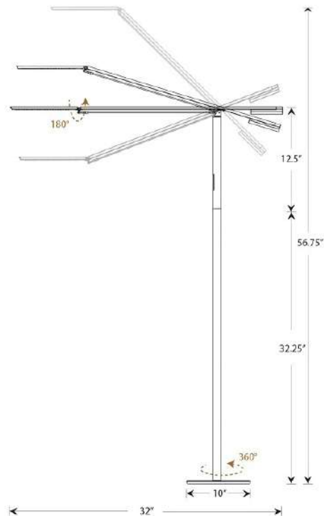
Horizontal and vertical reach
