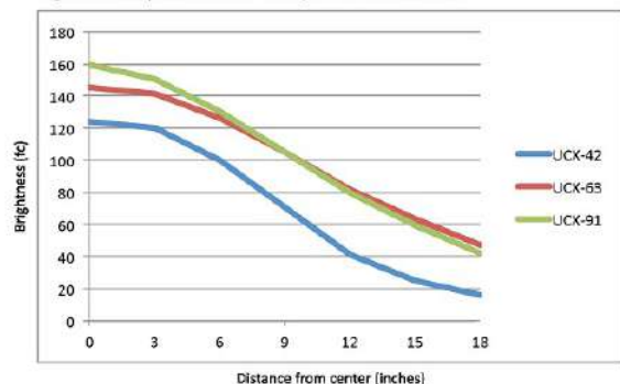
Light source placed at 18" away from worksurface
