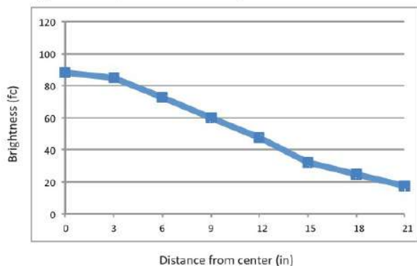
Light source placed at 15" away from worksurface
