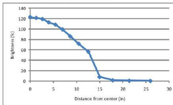
Light source placed at 15" away from worksurface
