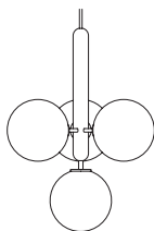
Miira 4 Design Sofie Refer Material Metal & Glass Dimensions ø380mm x 465mm Options Rock Grey/Optic Clear or Rock Grey/Opal White Technical Spechs G9, Dimmable
