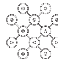
Liila 12 Wall/Ceiling Design Sofie Refer Material Metal & Glass Dimensions 845mm x 845mm Options Nordic Gold/Optic Clear or Nordic Gold/Opal White Technical Spechs G9, Dimmable
